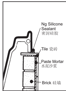
Hob Mount Tiling
