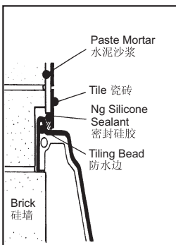
Rebated Into Wall
