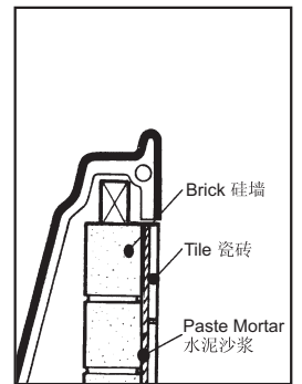
Flush Front Tiling
