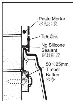
Packed Out From Wall
