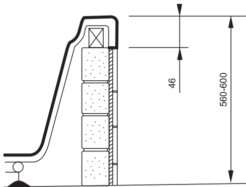
K-11221T-W03/K-11221T-H-*
