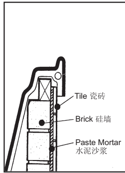
Under Flange Tiling
